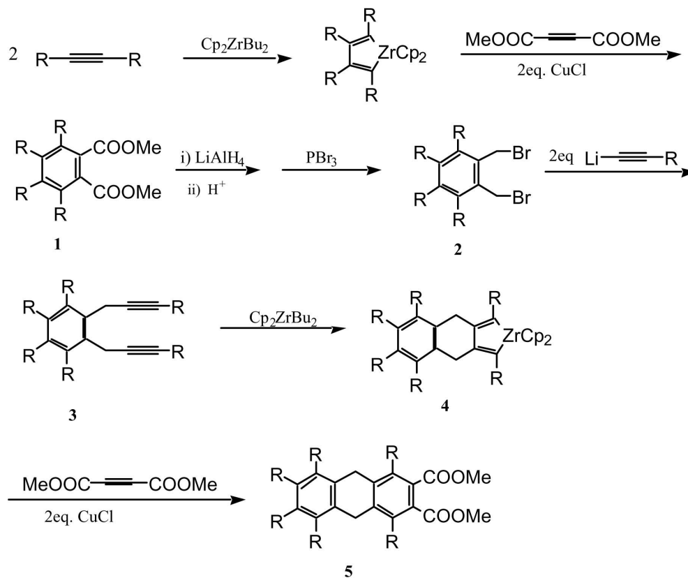
Scheme 1. Preparation of odd number ring compounds
